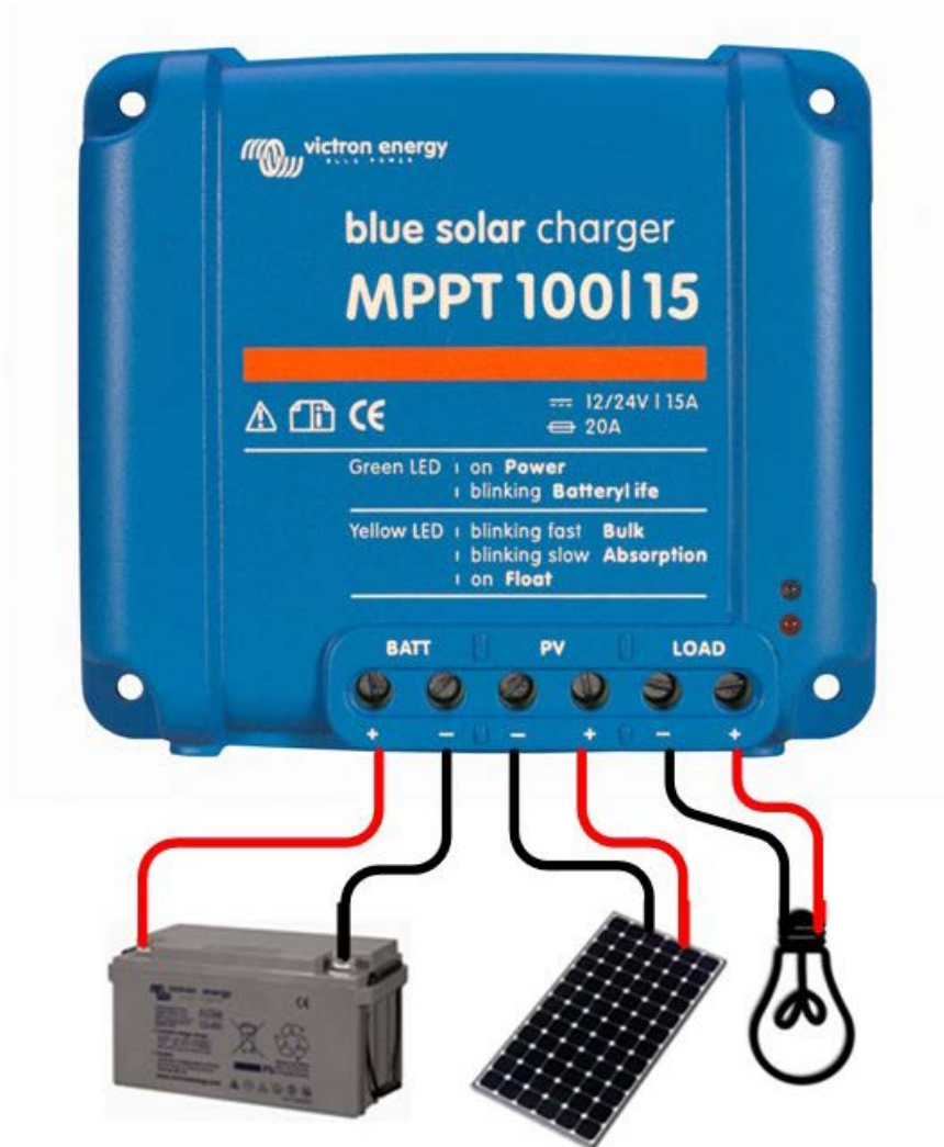
Figure 3: Power connections
